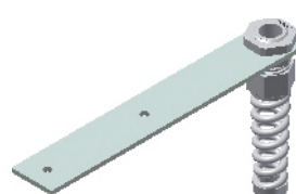
straight mounting bracket for spiral cable, 160x25mm incl. spiral cable gland M16 (roller shutters)
